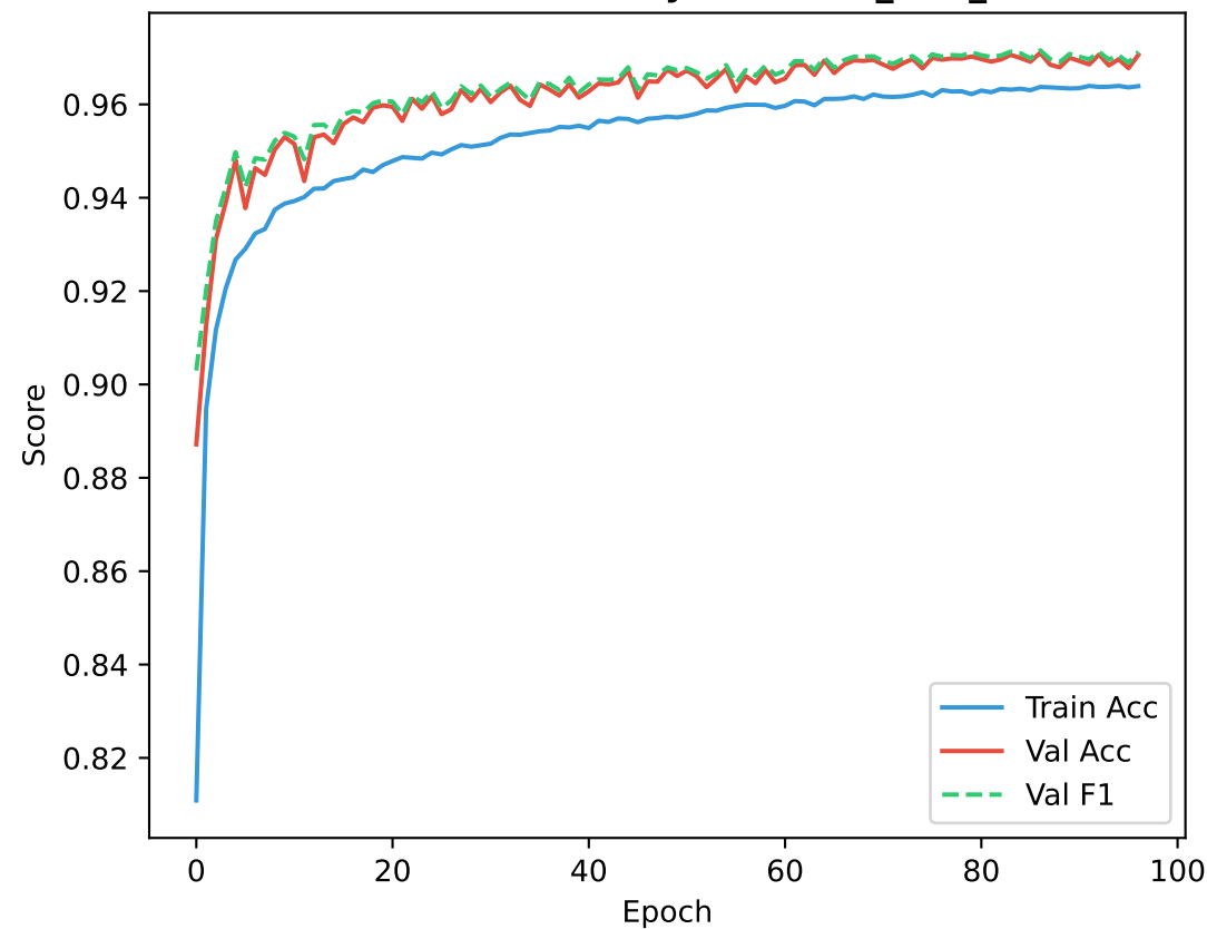
Transformer Accuracy/F1 — CIC_IIoT_2025
