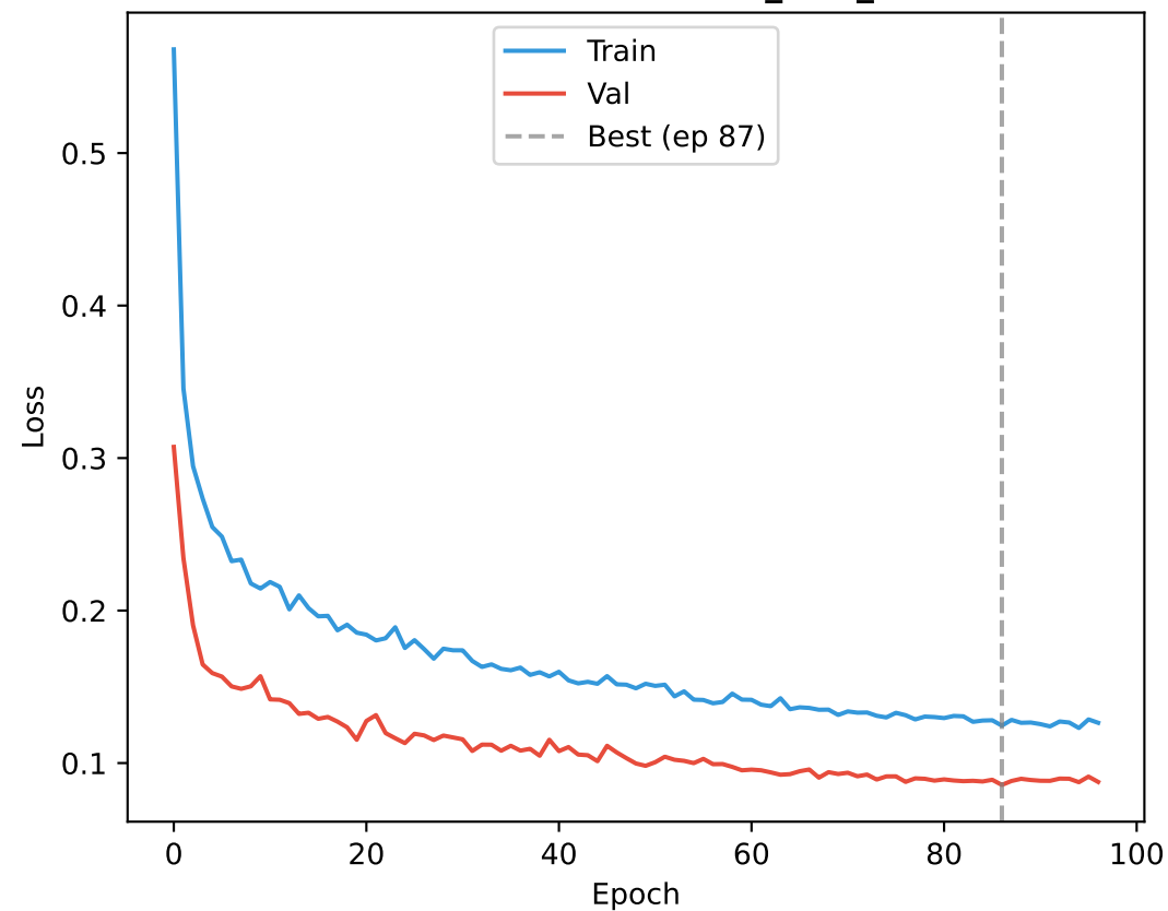
Transformer Loss — CIC_IIoT_2025
