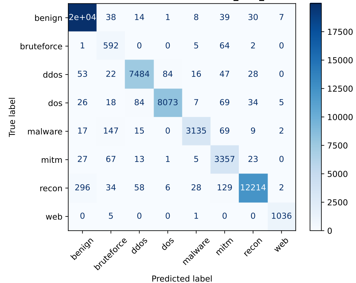
Transformer Confusion — CIC_IIoT_2025
